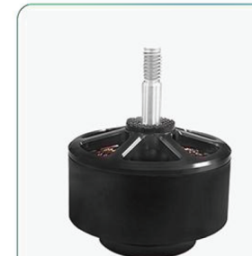
B4215 KV600 Dimension: \Phi 58.5 \times 52.8 mm Pulling force: 65/5199g
